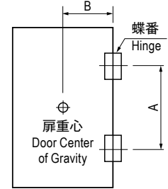
図1: 蝶番取付寸法図 (縦使い) Figure 1. Vertical use
