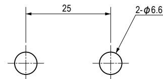
取付穴図 Hole for Installation
