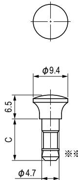
頭部形状No.5 Head Shape
