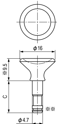
頭部形状No.1 Head Shape
