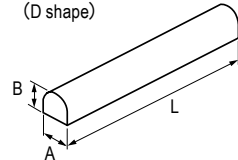
TM-98N-□ TM-98S-□ (カマボコ型) (D shape)
